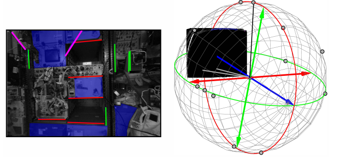
Fig. 8. Determination of the three vanishing points ( \mathbf{v}_1 , \mathbf{v}_2 , \mathbf{v}_3 ) in the Manhattan world. \mathbf{v}_1 is set as the plane normal vector. If the sampled line corresponds to the thick red line, the cross product of its normal vector (black) and \mathbf{v}_1 determines \mathbf{v}_2 . \mathbf{v}_3 is obtained by taking the cross product of \mathbf{v}_1 and \mathbf{v}_2 .
